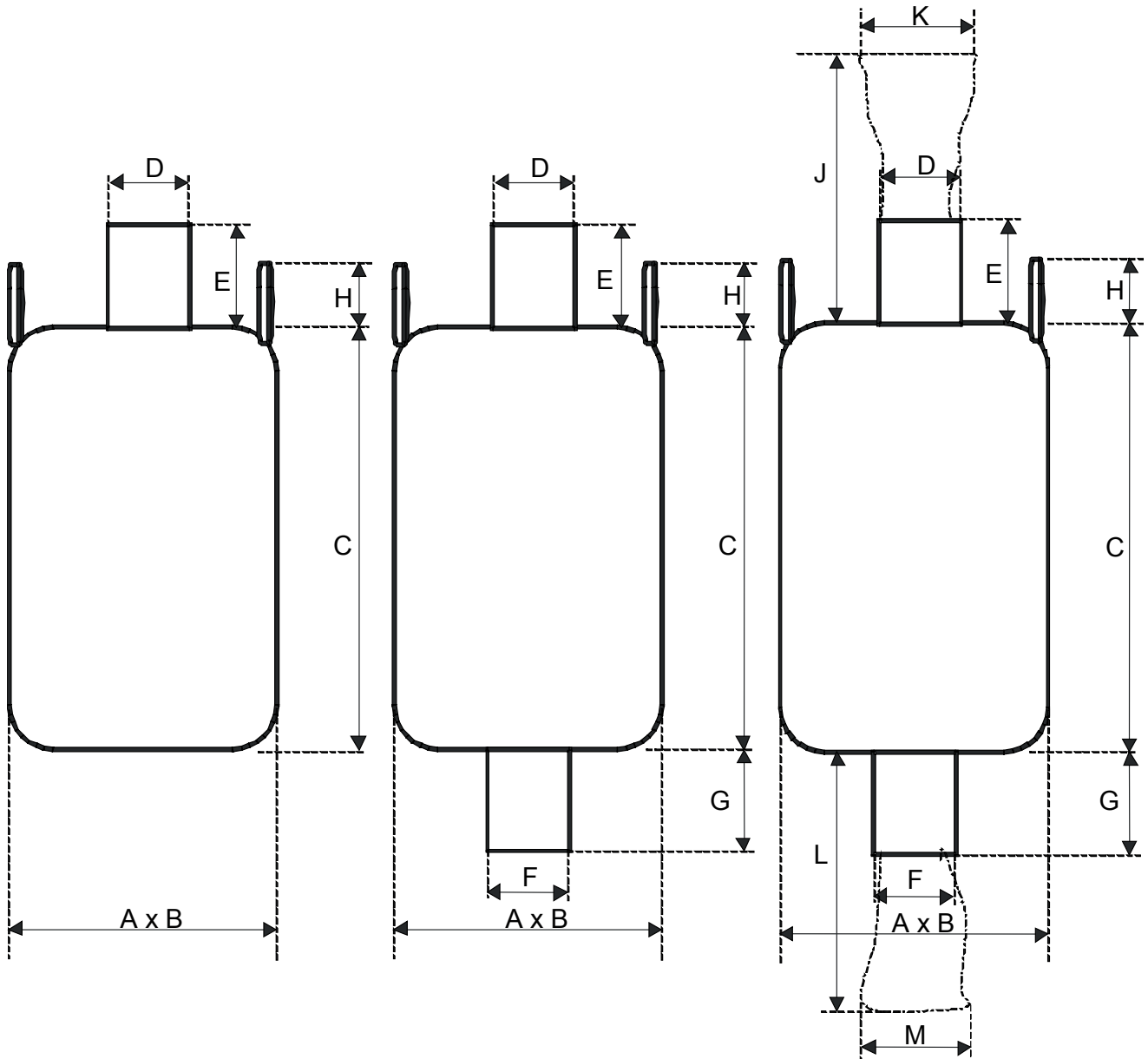
Single trip Big-Bag without outlet spout
